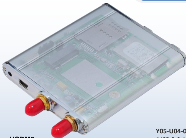
USBM2 (Wireless USB M.2 Card Adapter) x1 with MHF4-RPSMA RF cable 8cm x2
