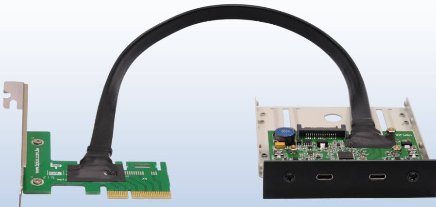
PP1142 (PCI Express to USB 3.1 Type C Front Drive Bay Docking System) x1
