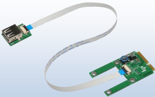
KZ-B34-USB (USB to MiniCard Extender) x1
