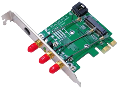
MP2W (Mini PCI-E / PCI-E Adapter ver 2.2) x1 with IPX to SMA / RP-SMA cable x3
