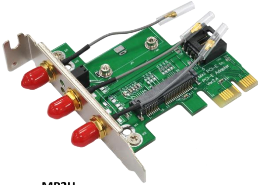
MP2H (mPCIe to PCIe adapter ver 2.4) x1 with IPX to SMA / RP-SMA cable x3
