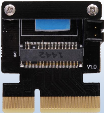
M2P4B PCIe 3.0 X4 to M.2 PCIe Gen3 SSD Adapter x1
